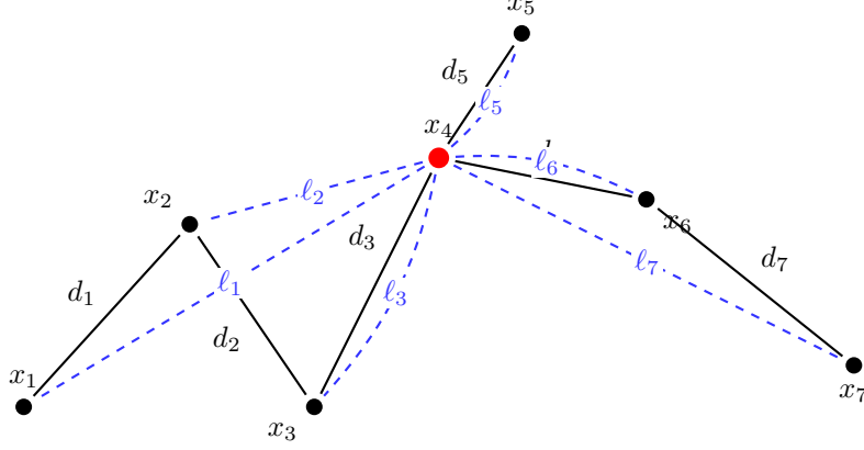
Fig. 2 Components of the proposed algorithm in 2D
