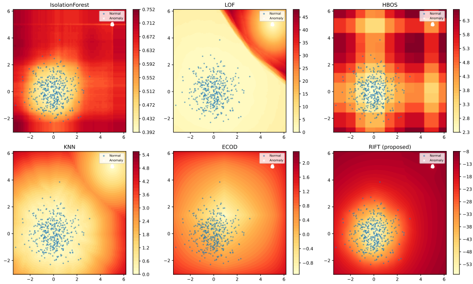
Fig. 6 Anomaly scores on the “clustered anomalies” dataset
