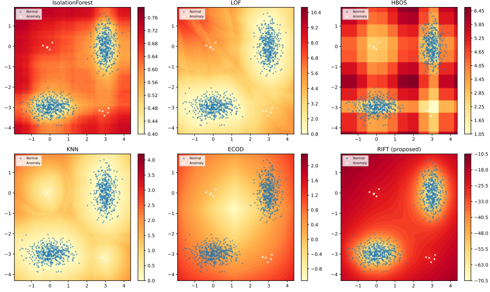
Fig. 4 Anomaly scores on the “blobs” dataset
