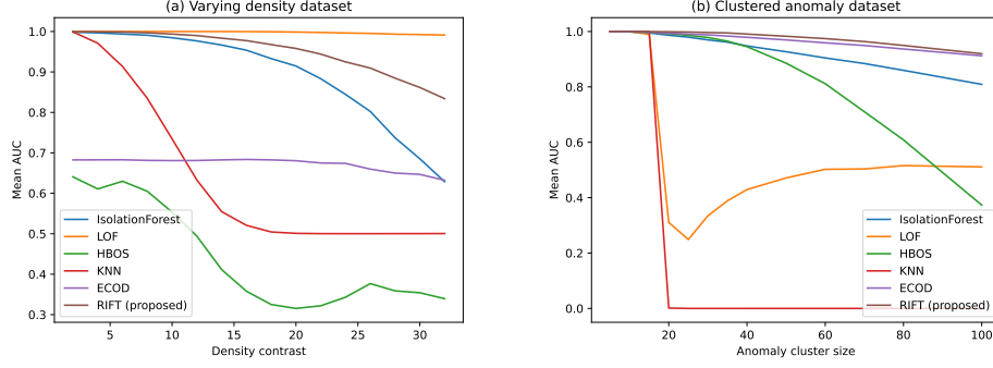
Fig. 7 Performance of anomaly detection methods on two synthetic datasets
