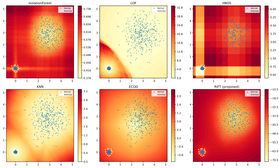
Fig. 5 Anomaly scores on the “varying density” dataset
