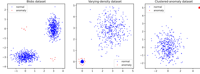
Fig. 3 Synthetic datasets used in the comparison
