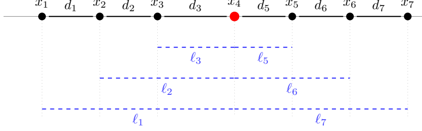
Fig. 1 Components of the explicit solution of the anomaly score for x_4
