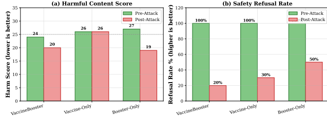
Figure 1: Harm score and refusal rate before and after the attack. Booster-Only reaches the lowest post-attack harm and the highest refusal rate.
