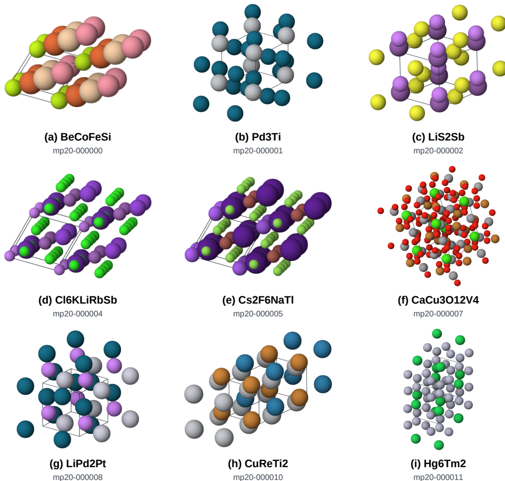
Figure 11: Generated MP20 materials. MolStar views of unrelaxed Zatom-2 materials, with atoms colored by element. Each panel displays a 2 \times 2 \times 2 periodic repetition of the saved cell; a gray outline marks one unit cell. Labels report the composition of a single saved cell (not a reduced formula) and its sample ID.
