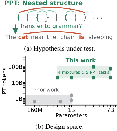
Figure 1: (a) PPT is claimed to induce a grammatical prior that transfers to natural language. (b) Prior work sits at or below 1B parameters and short training horizons. We span four scales, four PT mixtures, five PPT tasks, and up to 100B PT tokens.
