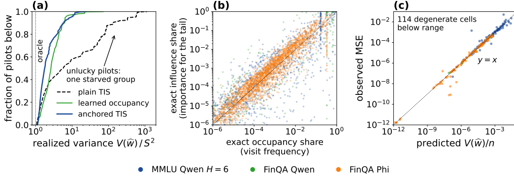
Figure 5: Anchoring reduces the variance penalty from poor pilots. (a) Realized/oracle leading variance; (b) occupancy versus tail-influence shares; (c) observed MSE versus the no-fit prediction V(w)/n . Rollouts are excluded.
