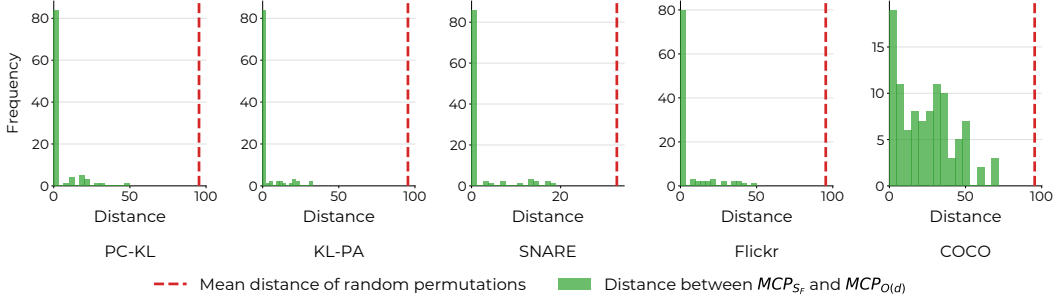
Figure 9: Extended validation of \text{MCP}_{O(d)} = \text{MCP}_{S_F} . Distance between \text{MCP}_{S_F} and the approximated \text{MCP}_{O(d)} (denoted as \tilde{P}_O ), computed on the anchors of the each dataset across 100 initializations. This figure complements Fig. 6 in the main text by demonstrating that the strict concentration at zero holds consistently across all evaluated domains, further validating Thm. 2.
