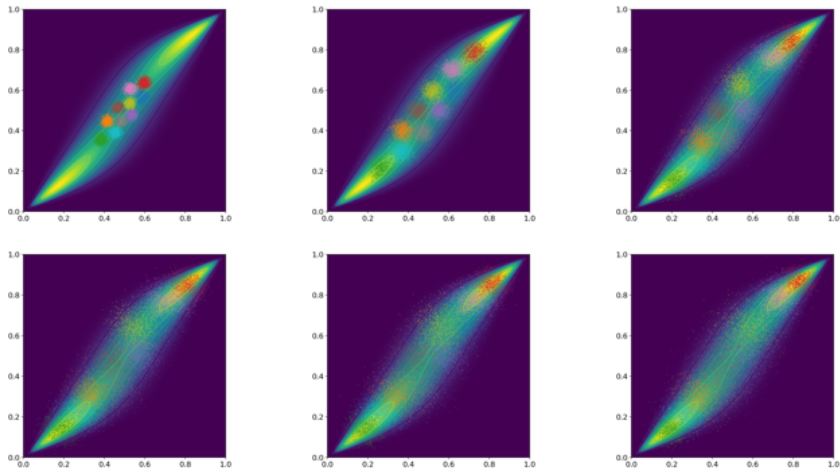
Figure 4.3.6: The evolution of the A = 10 variational mixture after 1k, 2k, 3k, 4k, 5k and 10k training iterations, respectively. The component mean parameters are randomly initialized around (0.5, 0.5) . The colored scatter points are samples from the different components with separate colors for each component.
