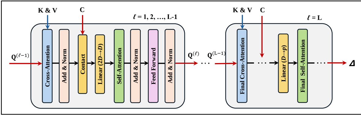
Fig. 2. Cross-self attention module structure. Left: the first L-1 layers, each at hidden width D (cross-attention to \mathbf{H} , coarse fusion as in Eq. (3), self-attention, and FFN). Right: the final ( L -th) layer follows the same high-level pipeline; the ellipsis inside the L -th block denotes submodules that are structurally identical to those in the preceding layers. In the last layer only, a linear layer maps from width D to width p before self-attention; the self-attention and FFN sublayers then run in the p -dimensional space. After the final FFN, the stack outputs \Delta for Eq. (4).
