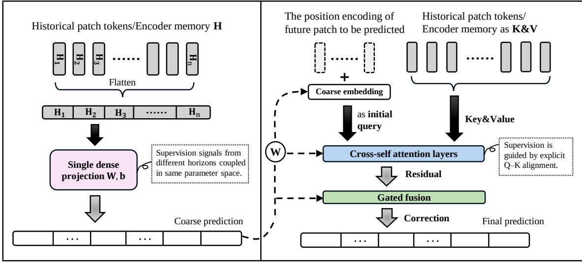
Fig. 1. Flatten readout vs. SACQ decoding. Left: flatten maps encoded historical memory to all future steps through one dense projection, sharing readout parameters across the horizon. Right: SACQ initializes coarse future-patch predictions, refines them with cross-self attention over historical memory, and merges a gated residual correction at each future patch. Details are given in Sec. III-C.
