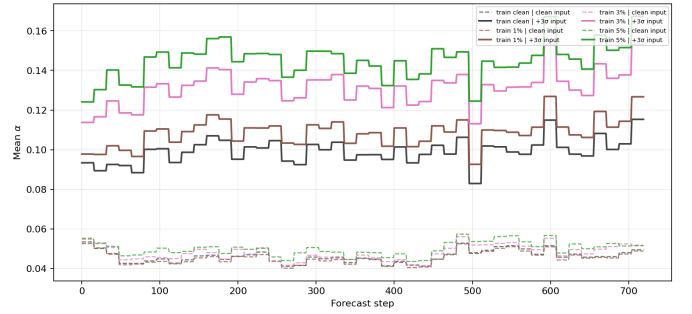
Fig. 5. Horizon-wise mean gate \alpha under clean versus spiked input histories ( +3\sigma on the lookback window). Dashed : clean test input. Solid : +3\sigma spiked test input. Colors index the training-set target-spike ratio (0%, 1%, 3%, 5%).
