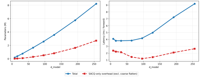
Fig. 7. Scaling with backbone width d_{\text{model}} . Left : parameter count (M). Right : forward-pass latency (ms). Blue solid: total model; red dashed: SACQ-only overhead excluding the coarse flatten map.
