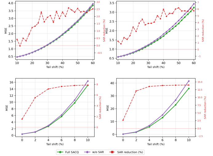
Fig. 4. SAR ablation under training-set tail shift. (a)–(b) ETTh1 at T_f=96 and 720. (c)–(d) Weather at T_f=96 and 720. Solid curves: full SACQ (with SAR) and w/o SAR; dashed curve: relative test-MSE reduction from SAR. Tail-shift rate increases the fraction of spike-corrupted supervision in the forecast tail during training only.
