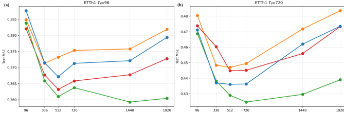
Fig. 6. Lookback sensitivity on ETTh1. Test MSE versus input length N for DLinear, PatchTST (flatten), SACQ+MSE, and SACQ+scaled log-cosh. (a) Short-horizon forecasting ( T_f=96 ): all methods improve when N grows from 96 to 336–512, then plateau. (b) Long-horizon forecasting ( T_f=720 ): SACQ+scaled log-cosh remains stable at N=1440 , whereas flatten baselines spike at the longest contexts.
