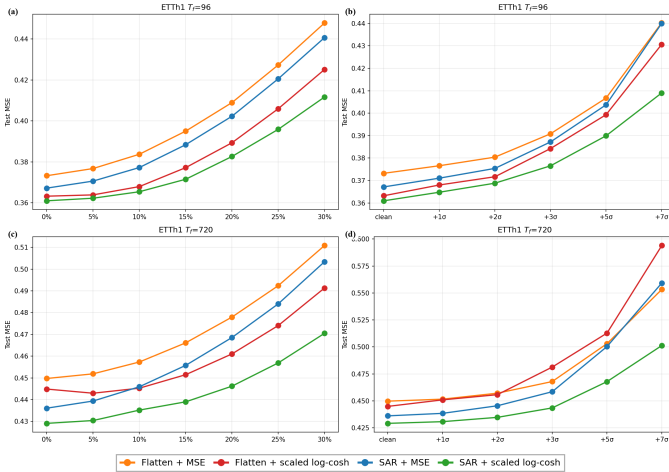
Fig. 3. Robustness on ETTh1 under training-set corruption. (a) T_f=96 , input masking: test MSE versus missing rate \rho on historical windows. (b) T_f=96 , target spikes: test MSE versus spike intensity (clean to +7\sigma_y ). (c)–(d) Same sweeps at long horizon T_f=720 . Curves compare Flatten+MSE, Flatten+scaled log-cosh, SAR+MSE, and SAR+scaled log-cosh; evaluation uses the clean test split.
