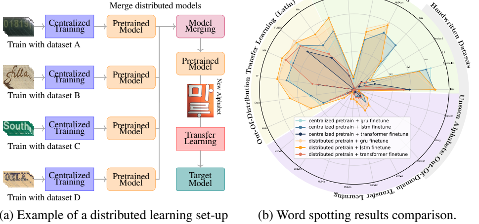
Figure 1: We show that distributed regimes (orange area, proposed) consistently outperform centralized pretraining (blue area) across a wide range of architectures and downstream tasks. We perform an extensive evaluation on 27 well-established Word Spotting and recognition datasets.
