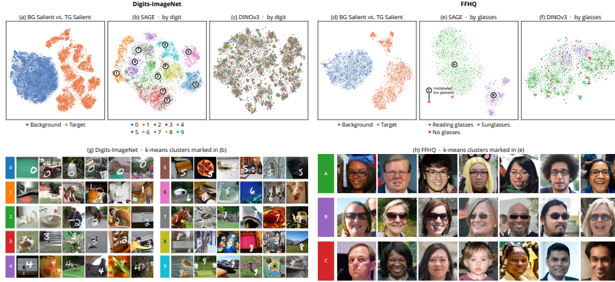
Figure 5: Subtype discovery in the salient space. Top: t-SNE of SAGE’s salient representations separates background and target images (a, d) and organizes digit and eyewear subtypes (b, e), whereas raw DINOv3 features mix them (c, f). Bottom: examples from the k -means clusters marked in (b, e) show coherent digit and eyewear groups (g, h); FFHQ cluster C contains images mislabeled as wearing glasses, and red points are audited no-glasses images.
