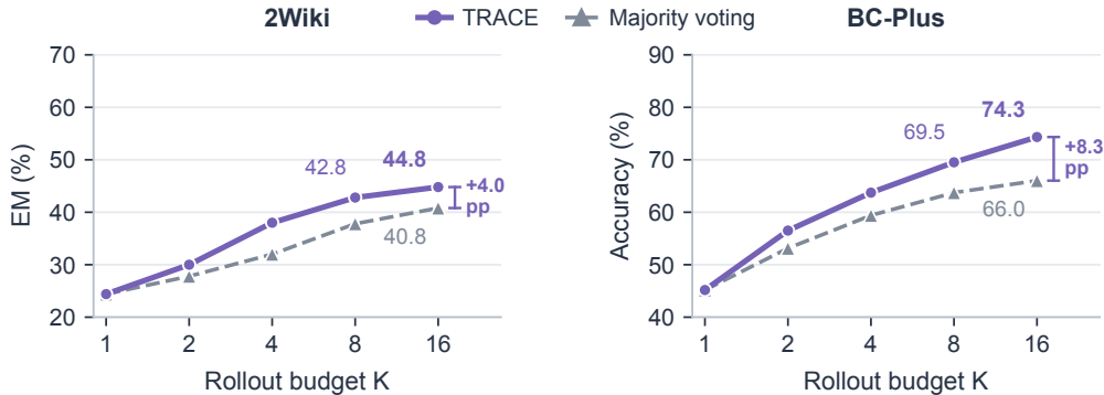
Figure 2: Final-answer performance with fixed TRACE checkpoints as the rollout budget increases. (a) 2Wiki EM with Qwen2.5-14B Base rollouts. (b) BrowseComp-Plus accuracy with gpt-oss-120B rollouts. Dashed curves show majority voting; brackets mark TRACE gains at K = 16 .
