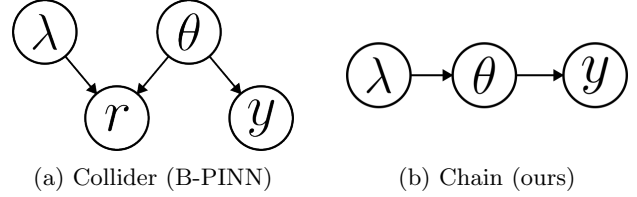
Figure 1: Modeling choices for physics-informed Bayesian inference. (a) Collider (B-PINN): Physics parameters \lambda and trajectory parameters \theta are a priori independent, interacting only when conditioned on equation residuals r . (b) Chain (ours): Physics \lambda directly generates trajectories \theta , which in turn generate data y .
