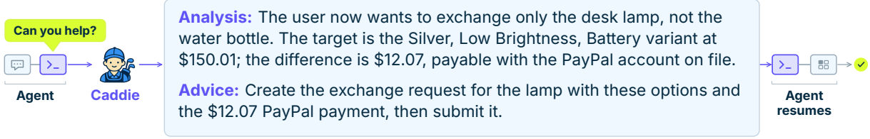
Figure 1. Training and using CADDIE. (a) Training: the frozen agent \pi_b rolls out a task and a step k is chosen randomly; at the prefix s_k the critic \pi_c^\theta samples G critiques; each critique is then appended to the prefix and the frozen agent rolls out N continuations until the end of the episode. The terminal rewards are normalized within the group and update only the critic with DAPO. (b) Inference: the agent decides when to consult the critic through the call_critic tool and receives the critique as the tool output.
