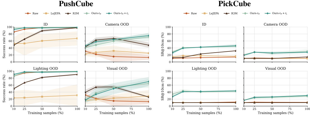
Figure 13: Sample efficiency of learned representations. Performance of different representations under varying amounts of training data on PushCube and PickCube, evaluated under ID and OOD settings.
