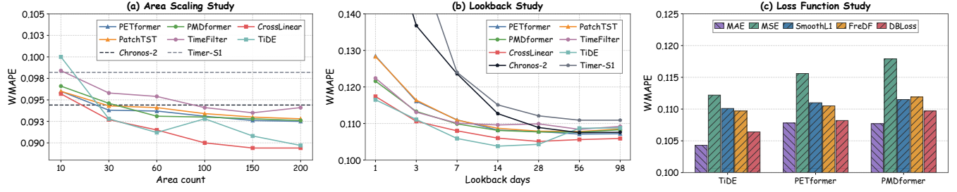
Figure 7: Studies on key benchmark design factors. (a) Effect of increasing the number of training areas while keeping the 10 target areas fixed. (b) Effect of varying the input lookback length. (c) Impact of different training losses.
