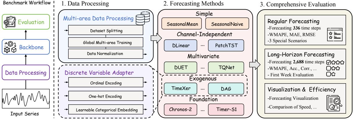
Figure 4: Overall architecture of RideBench. The left illustrates the general benchmark workflow, and the right demonstrates the detailed implementation details.
