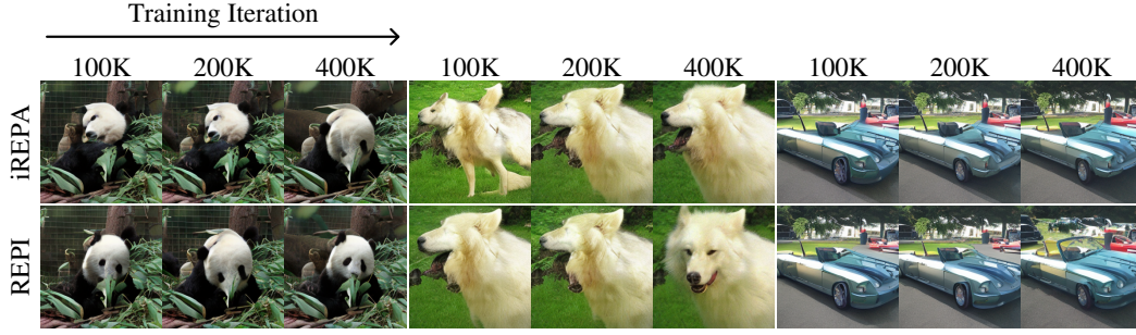
Figure 3: Qualitative comparison across training iterations. Generated samples from SiT-XL/2 trained with iREPA (top) and REPI (bottom) over the first 400K iterations. Both models use the same initial noise and sampler, without classifier-free guidance.
