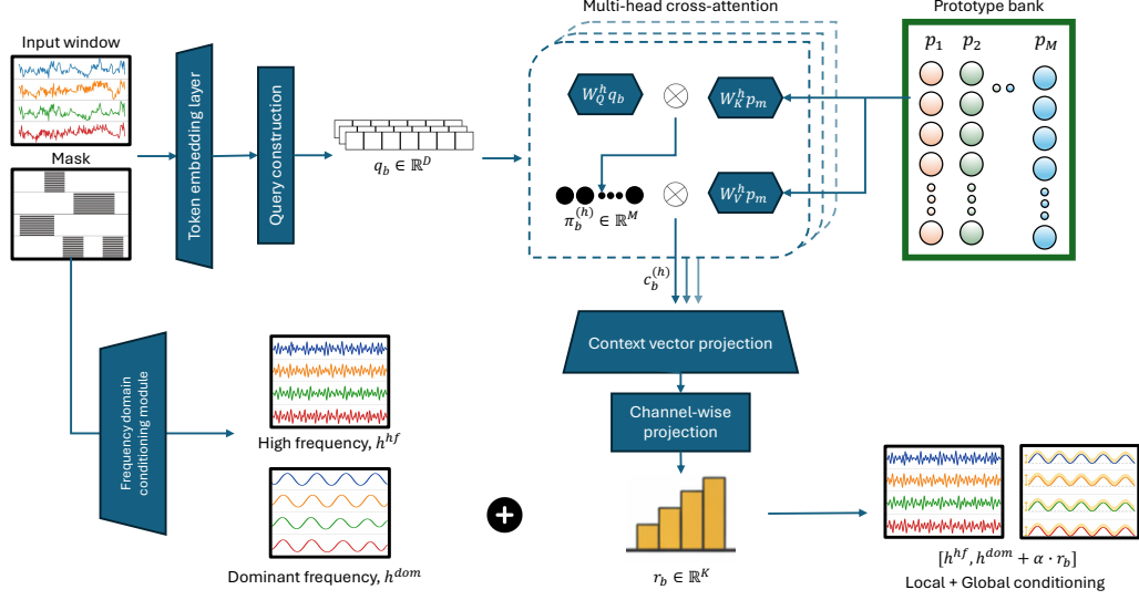
Figure 2: Prototype-conditioning module
