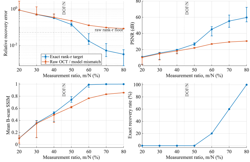
Fig. 4 The first three panels show medians over ten balanced random starts, with error bars spanning the 25th to 75th percentiles. The dashed horizontal line is the rank-3 approximation floor of the untruncated target. The vertical line (DOF/N) at r(n_1 + n_2 - r)n_3/N = 0.4420 is only a parameter-count reference, not a theoretical phase-transition threshold. The lower-right panel shows the percentage of successful starts for the exact-rank target.
