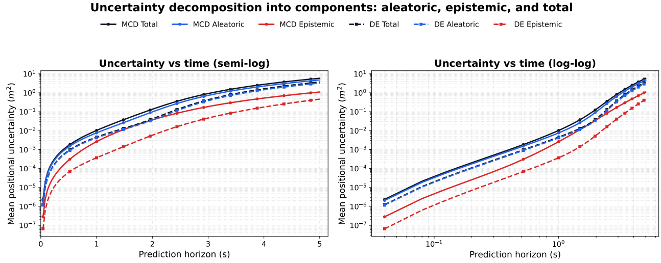
Figure 9: Decomposition of trajectory space predictive uncertainty (different scales) into aleatoric, epistemic, and total components for X-TRACK-MCD and X-TRACK-DE.
