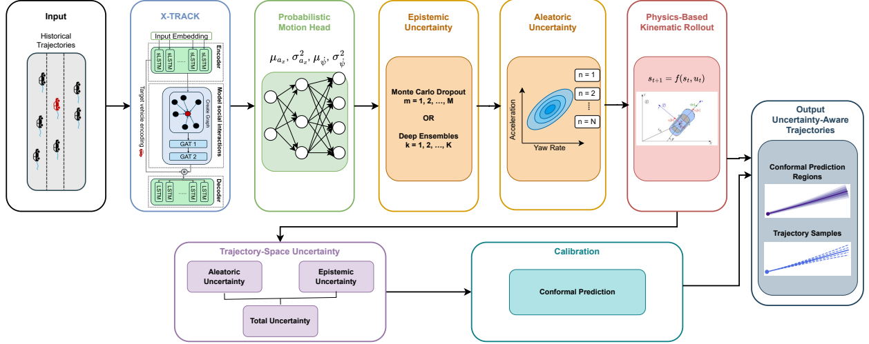
Figure 1: Overview of the uncertainty-aware X-TRACK framework. Aleatoric uncertainty is estimated by sampling from the predicted motion distributions, and epistemic uncertainty is obtained using MC Dropout or Deep Ensembles. The sampled vehicle motion variables are propagated through the physics-based kinematic layer to obtain uncertainty in trajectory space. To obtain calibrated trajectory uncertainty regions, conformal prediction is applied.
