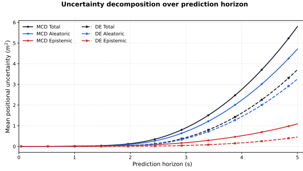
Figure 3: Decomposition of uncertainty into individual components for both variants.
