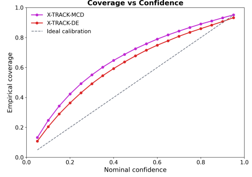
Figure 4: Comparing empirical coverage and nominal confidence for raw predictive distributions of X-TRACK-MCD and X-TRACK-DE.
