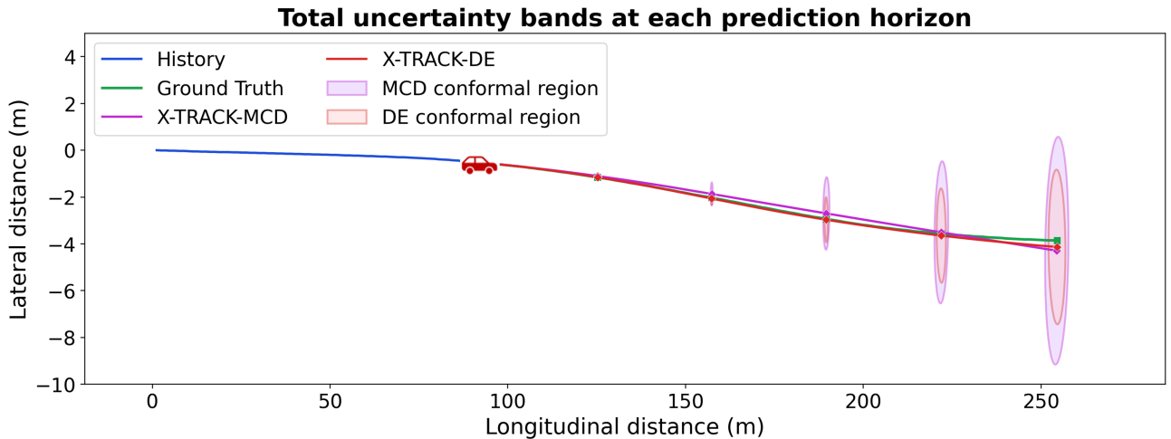
Figure 5: Comparison of total predictive uncertainty for X-TRACK-MCD and X-TRACK-DE over different prediction horizons.
