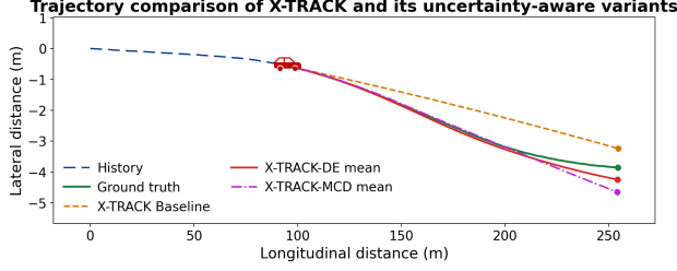
Figure 2: Qualitative comparison of ground truth with deterministic X-TRACK and predictive means of X-TRACK-MCD and X-TRACK-DE.
