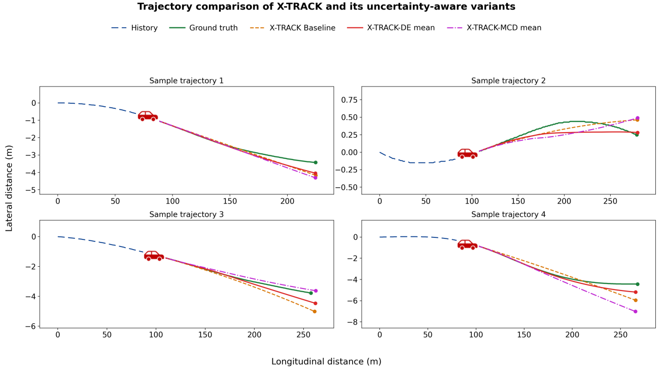
Figure 8: Qualitative comparison of ground-truth trajectories with deterministic X-TRACK and the predictive means of its uncertainty-aware variants.
