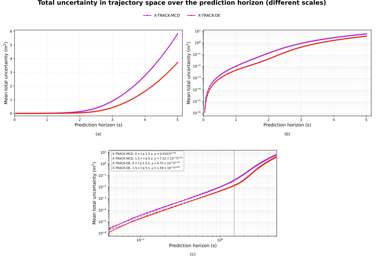
Figure 6: Total predictive uncertainty in trajectory space over the prediction horizon for X-TRACK-MCD and X-TRACK-DE. The same mean uncertainty is shown using (a) linear, (b) semi-logarithmic, and (c) log-log scales.
