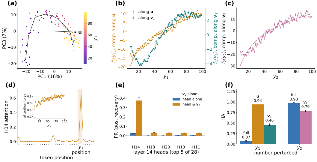
Figure 2: A single causal direction for numbers controls model comparison. (a) A causal direction \mathbf{u} found in Layer 13’s residual stream causally affects model behavior, despite the presence of curved geometry in the activations, as observed in principal components 1, 3. (b, c) Projection of activations onto the obtained causal directions \mathbf{u} , \mathbf{v}_1 , \mathbf{v}_2 encode the number magnitude for a wide range of values. While \mathbf{u} is in layer 13 residual stream at the first number y_1 ’s position, \mathbf{v}_1 , \mathbf{v}_2 are causal directions encoding y_1 , y_2 resp. at y_2 ’s position. \mathbf{v}_1 is obtained using DAS at an attention head H14’s outputs. (d) Attention head 14 in layer 14 attends to the position of the first number y_1 , irrespective of the number value, serving as a copy head. (e) Among all the attention heads in Layer 14, head H14 is causally involved in the model’s computation, showing significantly higher position recovery than others. (f) Patching along \mathbf{u} , \mathbf{v}_1 , \mathbf{v}_2 has significant causal effects on model behavior, as shown by interchange intervention accuracy (IIA).
