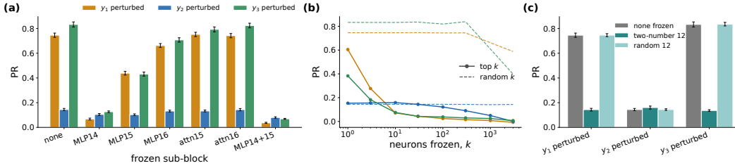
Figure 31: Position recovery of the patch of the span of \mathbf{v}_1, \mathbf{v}_2, \mathbf{v}_3 in the pre-MLP layer-14 residual at the position of y_3 , by perturbed number, while parts of the network are frozen. (a) One sub-block’s output at the position of y_3 frozen to its corrupted value. (b) The top k neurons by this task’s attribution ranking (solid) or k random neurons (dashed) frozen. (c) No neurons frozen, the 12 shared neurons of the two-number task frozen, and 12 random neurons frozen.
