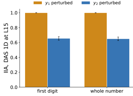
Figure 38: IIA of the rank-one direction in the layer-15 residual at the position of y_2 , fitted with y_1 perturbed and evaluated in both cases, scored on the first generated token and on the whole generated number, as in Figure 36.
