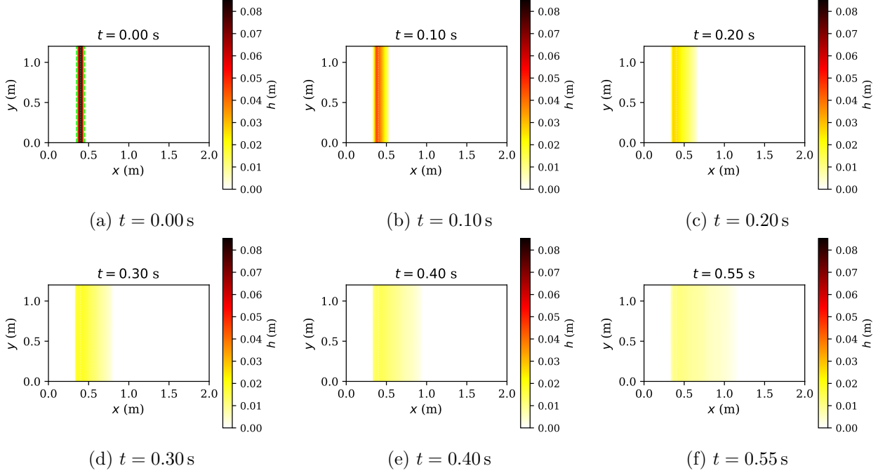
Figure 29: Pseudo-2D case, \zeta = 30^\circ : top-view depth contours at six time instants. Contour levels are identical across all panels.
