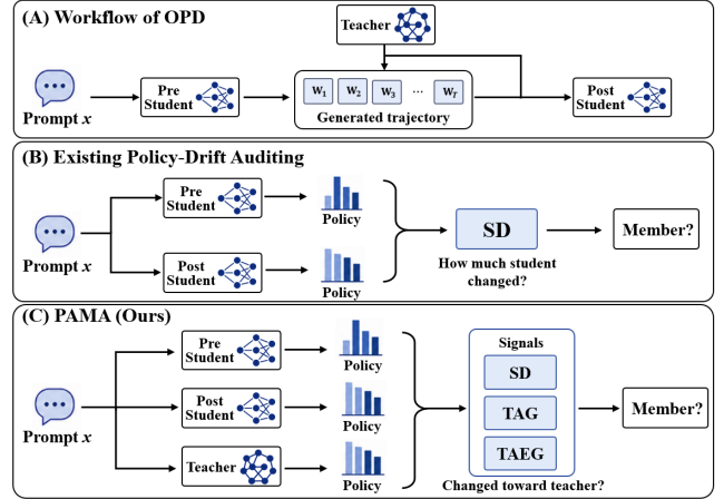
Figure 1: Overview of OPD prompt and membership auditing: (A) teacher-guided student training, (B) policy-drift auditing, and (C) PAMA with teacher-directed alignment.
