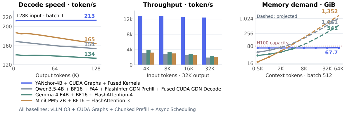
Figure 2. Single-H100 inference: sustained decoding speed, higher batched throughput, and bounded memory demand. Left: cumulative decode speed. Middle: end-to-end output throughput, selecting the batch size with the highest measured throughput for each model and input length. Right: batch-512 peak memory demand; solid curves use measured components, dashed curves project KV growth, and the dotted line marks device capacity. Appendix D gives the workloads and runtime settings.
