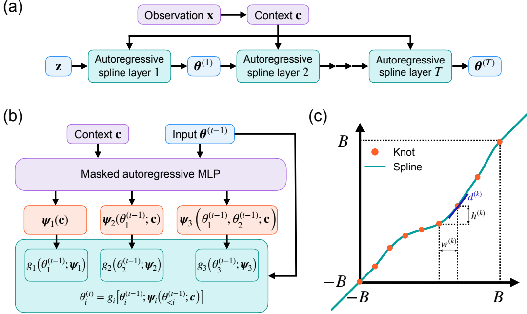
FIG. 8. Neural spline flow architecture. (a) A base sample \mathbf{z} is transformed through T autoregressive spline layers into a posterior parameter sample \theta^{(T)} , with each layer conditioned on the context \mathbf{c} derived from the observation \mathbf{x} . (b) Structure of an autoregressive spline layer, illustrated for three coordinates. A masked autoregressive MLP generates the spline parameters \psi_i from the preceding coordinates \theta_{<i}^{(t-1)} and the context \mathbf{c} . The scalar transforms g_i then map each input coordinate to \theta_i^{(t)} . (c) A monotonic rational-quadratic spline illustrated with K+1=9 knots, specified by bin widths w^{(k)} , heights h^{(k)} , and knot derivatives d^{(k)} , with identity tails outside [-B, B] .
