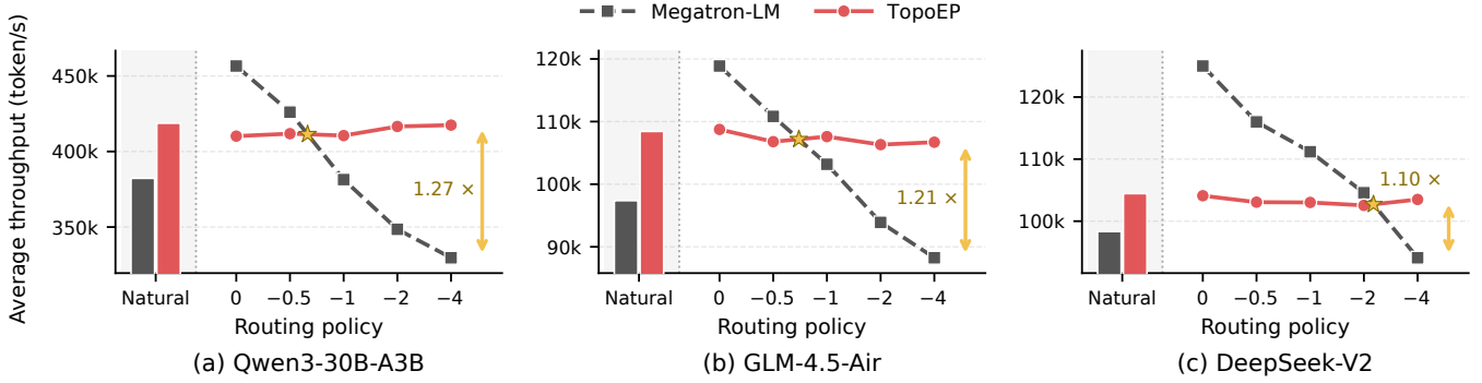
Figure 12: Average end-to-end training throughput under natural and synthetic routing. The synthetic settings vary router_skew from 0 to -4. Stars mark interpolated throughput crossovers, and double-headed arrows show the TopoEP /Megatron-LM throughput ratio at router_skew = -4.
