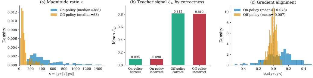
Figure 7: On-policy versus off-policy semantic conflict. On-policy distillation has a higher median \kappa but fewer incorrect trajectories with genuinely opposed reward and distillation gradients; off-policy supervision reverses this pattern.
