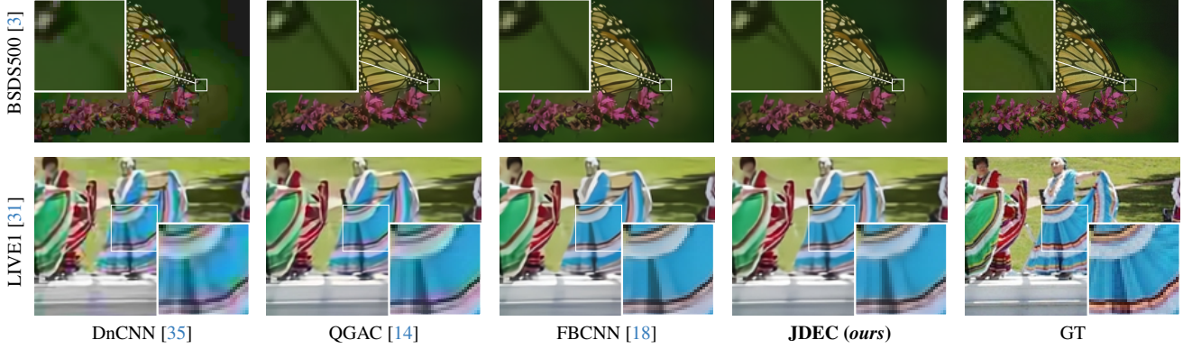
Figure 7. Qualitative comparison in color JPEG artifact removal ( q = 10 ).
