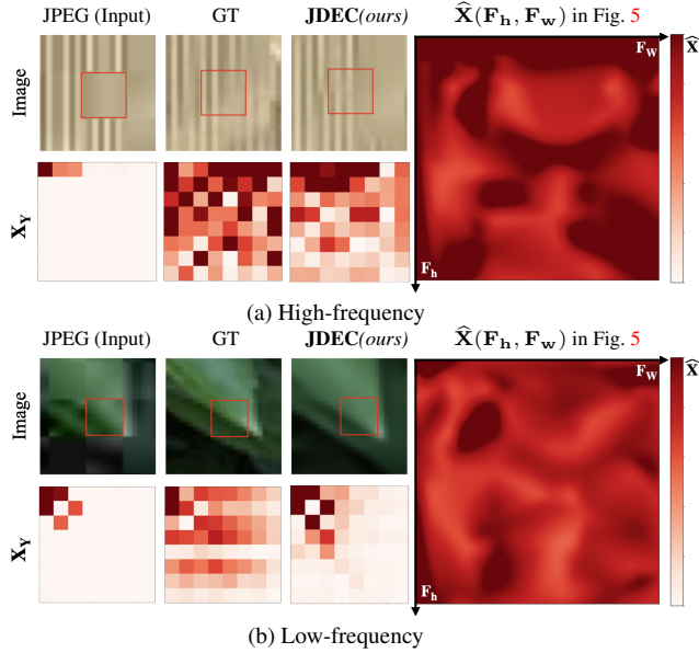
Figure 10. Comparison of the estimated spectra of the Continuous Cosine Formulation (CCF). The quality factor of input is 10. The estimated CCF spectrum follows the spectrum of ground-truth images despite severe distortion.
