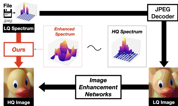
Figure 1. Overall concept of proposed JPEG decoding Instead of using a conventional JPEG decoder to refine the high-quality (HQ) image from the low-quality (LQ) image, our JDEC directly decodes the LQ spectrum by learning a continuous spectrum.
