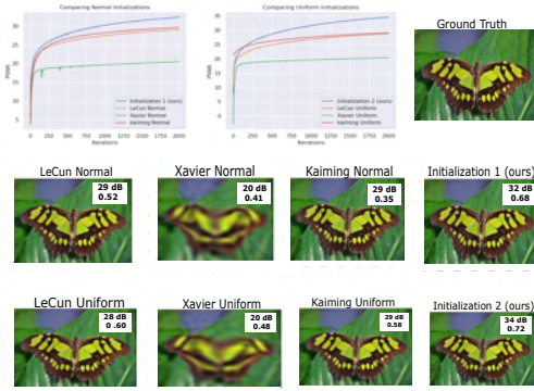
Figure 5. The figure shows the results for a 4\times single image super resolution with four normal initializations and four uniform initializations. Networks initialized with initialization 1 (our) and initialization 2 (our) produced the highest train dB and SSIM at convergence. Zoom in for better viewing.
