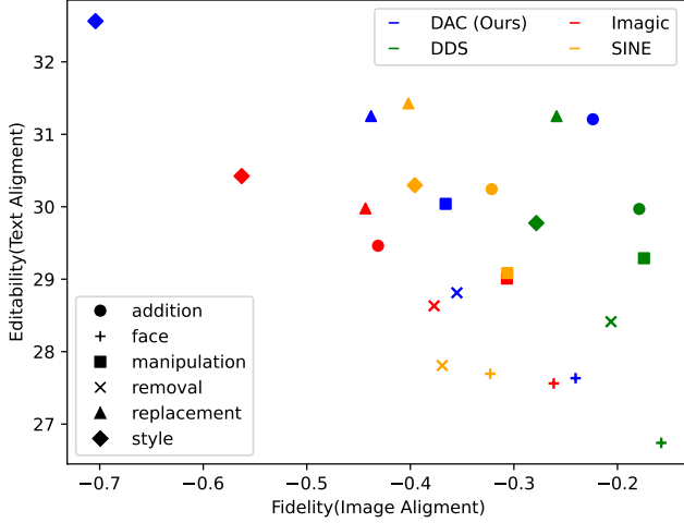
Figure 8. Image Alignment: minus LPIPS. Text Alignment: CLIP-score. Both values are the larger the better.
