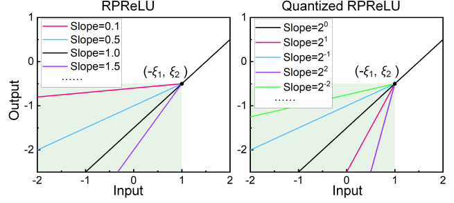
Figure 5. The slope of RPRReLU can be any continuous value greater than 0, while the slope of the proposed quantized RPRReLU is only allowed to be an integer power of 2.
