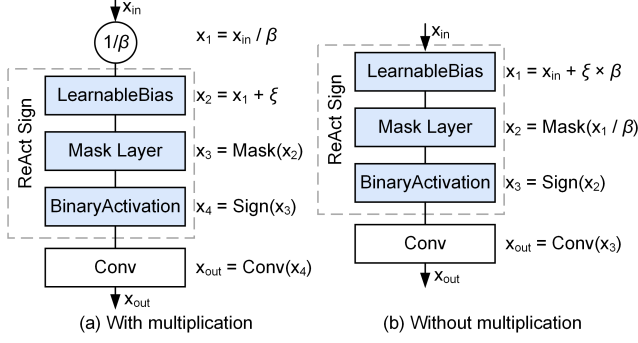
Figure 4. (a) The original structure with multiplication. (b) The equivalent structure, although transforming one multiplication operation into two, can both be eliminated.
