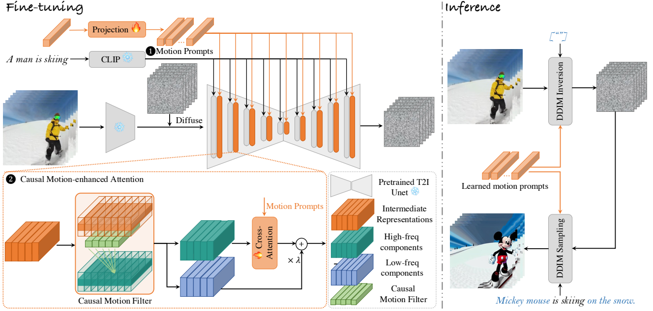
Figure 2. The overall of CAusal Motion Enhancement for Lifting text-driven video editing, consisting of ❶ Motion Prompt Learning and ❷ CAusal Motion-enhanced Attention (CAM-Attn) . The synergistic interaction between the two components is pivotal in enhancing motion coherence, concurrently preserving the generalization of appearance content across various textual prompts. During inference, the learned motion prompts function as a motion condition, and work synergistically with the textual condition for the denoising process.
