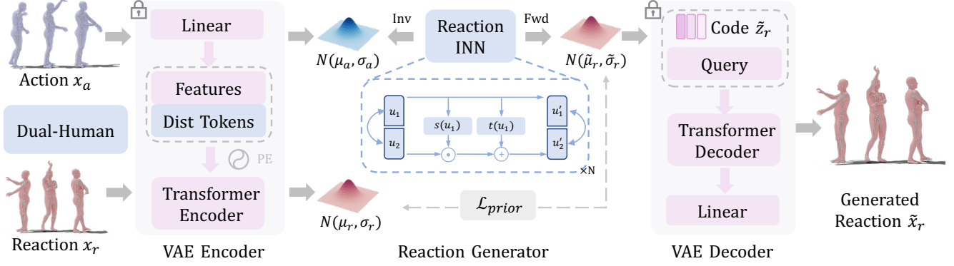
Figure 3. Reaction Priors. The reaction priors are composed of a VAE encoder, a reaction generator, and a VAE decoder. Initially, the VAE encoder maps the motion to the latent distribution. After that, the action distribution \mathcal{N}(\mu_a, \sigma_a) is fed to the reaction generator and converted to the reaction distribution \mathcal{N}(\tilde{\mu}_r, \tilde{\sigma}_r) , which are then recovered to the generated reaction.
