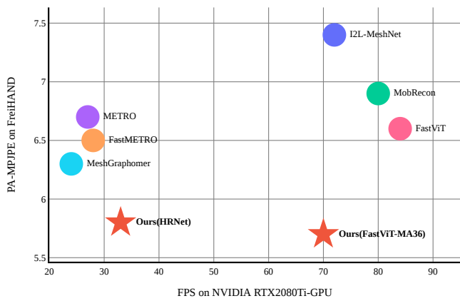
Figure 1. Trade-off between Accuracy and Inference Speed. Our technique surpasses non-real-time methods ( \leq 40 fps) in both speed and precision. Compared to real-time methods ( \geq 70 fps), it offers a substantial boost in accuracy while preserving comparable speeds. For fair comparison, all speed evaluations were conducted on a 2080ti GPU with a batch size of one.
