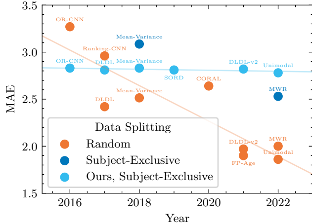
Figure 1. Mean Absolute Error (MAE) ↓ of age estimation methods on the MORPH dataset, as reported in the existing literature and measured by us, viewed over time. Random splitting remains the prevalent data splitting strategy. The consistent performance improvements over time are attributed in the literature to specialized loss functions for age estimation. Subject-exclusive (identity-disjoint) data splitting is rarely employed. With unified subject-exclusive data splitting and all factors except the loss function fixed, all evaluated methods yield comparable results, failing to achieve the performance gains promised by the random splitting.
