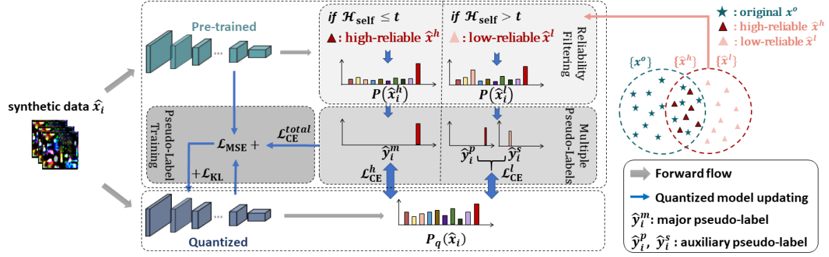
Figure 3. The framework of the proposed method. In the proposed method, synthetic data is evaluated with self-entropy of the pre-trained network on the synthetic data, which is divided into high- and low-reliable data. Then, the multiple pseudo-labels are used to label the evaluated synthetic data according to its reliability. The high-reliable samples are assigned with major pseudo-labels, and the low-reliable samples use auxiliary pseudo-labels. With these multiple pseudo-labels, the pseudo-labels cross-entropy loss can be obtained and combined with the MSE loss function to guide the quantized network has similar prediction ability with pre-trained network.
