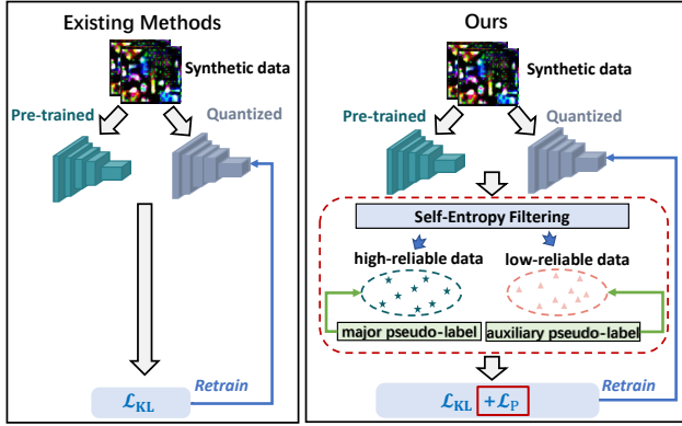
Figure 2. The difference between existing data-free methods and our method. The existing methods optimize the quantizer or retrain the pre-trained network with quantization constraint directly without evaluating the synthetic data. We propose to evaluate the synthetic data with self-entropy and divide the synthetic data into high- and low-reliable datasets before training the quantized network for better performance.
