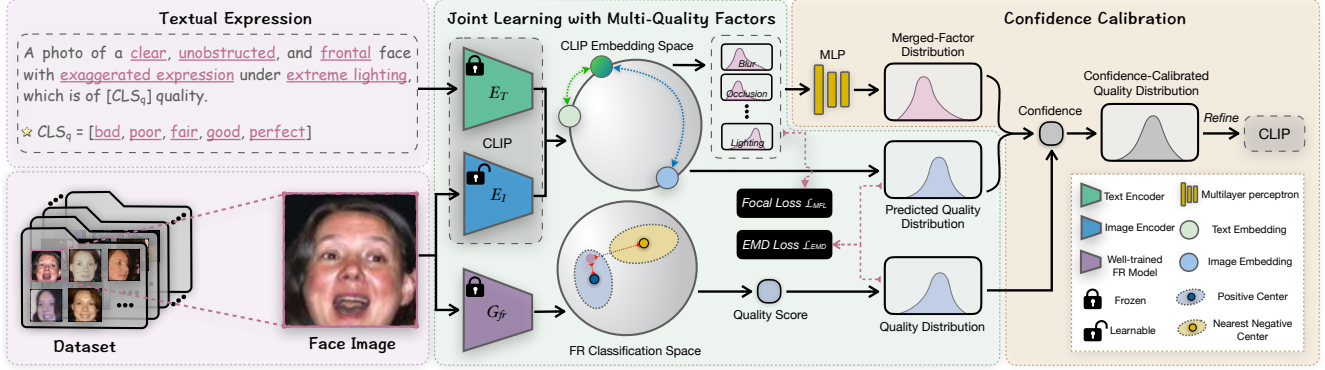
Figure 2. Illustration of the overall framework of the proposed CLIB-FIQA. Specifically, a face image along with its corresponding textual expression of quality factors are processed through the CLIP model. Then, the output is decomposed into the joint distribution of the quality factor and the predicted quality distribution. Herein, we leverage the joint learning strategy, enabling the classification information of quality factors to aid in fitting the quality distribution derived from the Face Recognition (FR) model. In the subsequent stage, to calibrate the confidence of the quality distribution, we use a Multilayer Perceptron (MLP) to transform the joint distribution of quality factors into a merged-factor distribution. The confidence is then computed based on the distance between the merged-factor and predicted quality distributions. Finally, the confidence-calibrated quality distribution is leveraged to refine the model in order to solve the fitting bottleneck caused by the uncertain quality supervision from the FR model. In the inference phase, an image of a face and the total possible textual expressions are fed into the CLIP for quality prediction.
