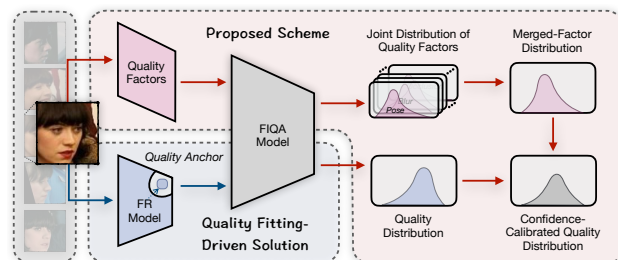
Figure 1. Illustration of the core idea of previous and the proposed FIQA schemes. Previous Quality Fitting-Driven Solution only considers the quality anchor provided by the dependent Face Recognition (FR) model. Our Proposed Scheme engages various quality factors to both facilitate the training of the FIQA model and calibrate the confidence of the quality distribution.
