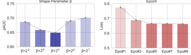
Figure 4. Parameter sensitivity for the shape parameter (left) and the number of epochs (right) in the first training stage.
