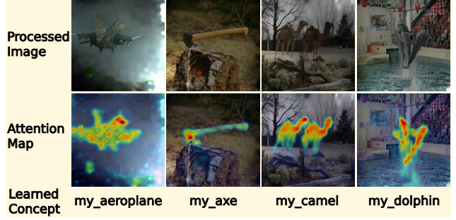
Figure 5. Attention maps for learned concepts on processed images.
