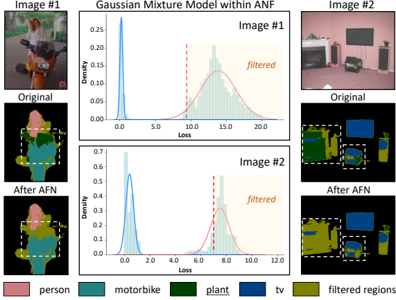
Figure 4. The loss distribution of images with noisy pseudo-labels. The model produces incorrect pseudo-labels of plant . Two peaks appear in the loss distribution on the two pseudo-labels, and the red peak with anomalous losses is mainly caused by noises. The distribution of normal losses is rescaled for visualization.
