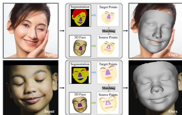
Figure 1. We introduce Part Re-projection Distance Loss (PRDL) for 3D face reconstruction, leveraging the geometric guidance provided by facial part segmentation. PRDL enhances the alignment of reconstructed facial features with the original image and excels in capturing extreme expressions.
