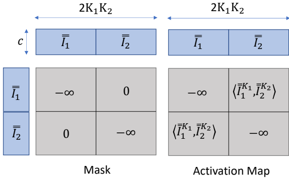
Figure 3. Computing the cross-attention using a Transformer-Encoder and the input mask, M . The mask M zeros the self-attention terms, retaining only the cross-attention terms.
