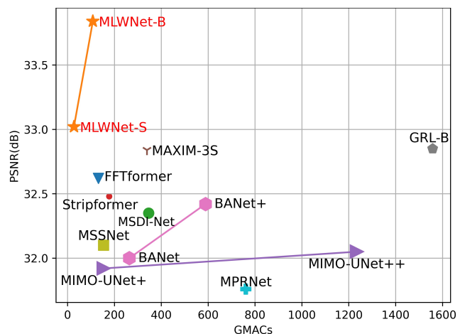
Figure 1. Performance comparison on the RealBlur-J [23] test dataset in terms of PSNR and GMACs. Our proposed MLWNet achieves superiority in comparison with other state-of-the-arts.
