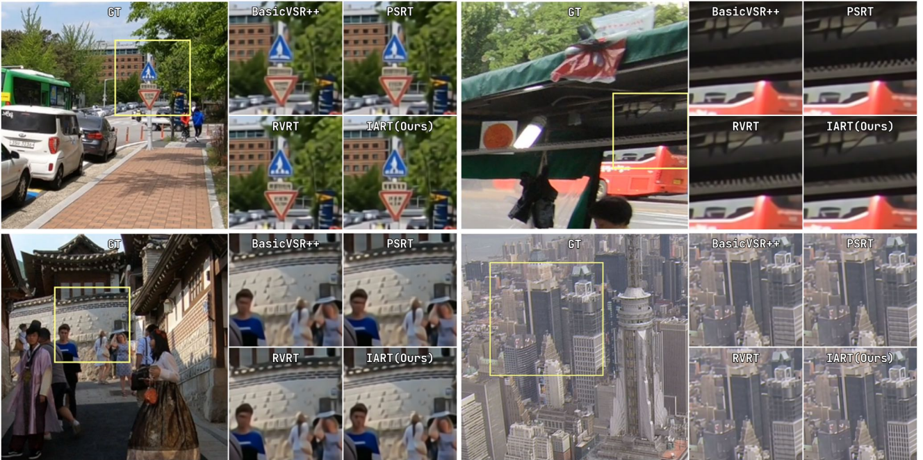
Figure 5. Qualitative comparisons on REDS4 and Vid4. IA-RT provides sharper results and more fine-grained patterns.
