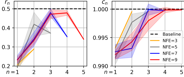
Figure 7. The learned coefficients r_n and c_n vary in different steps and the mean values are consistently lower than the default setting.
