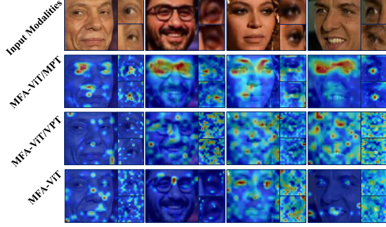
Figure 5. Visualization of activation maps for MFA-ViT with MPT, VPT, and no prompt strategies.
