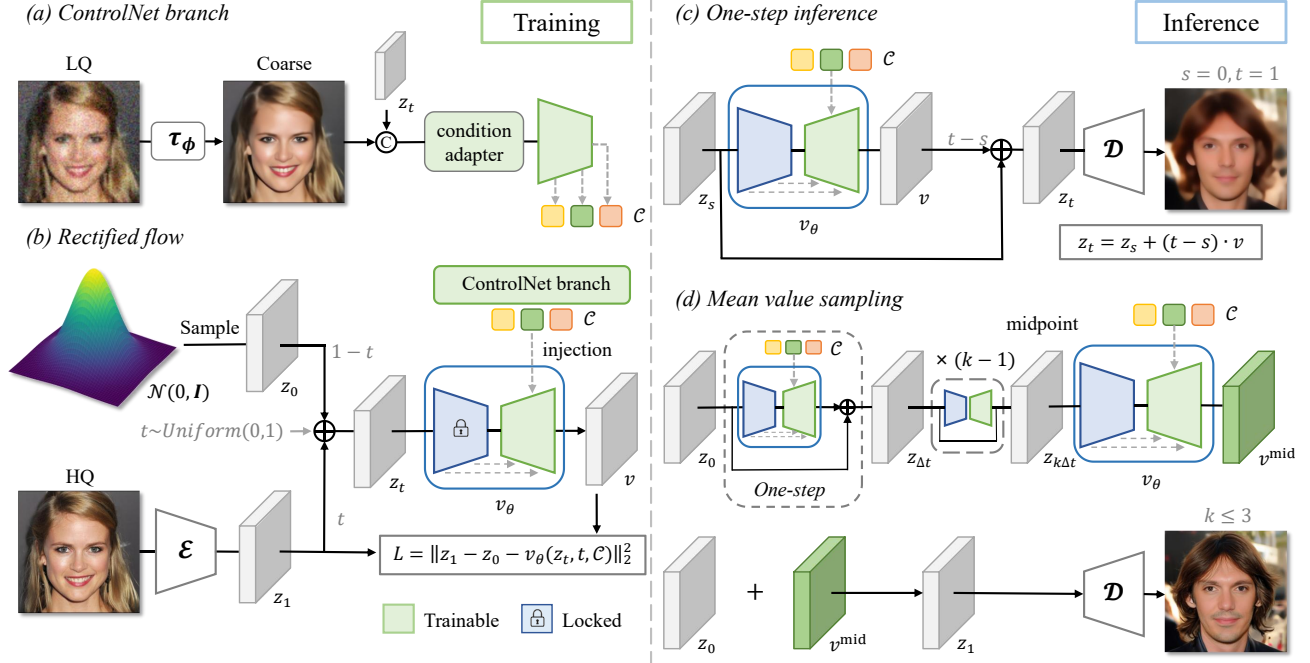
Figure 3. The overall framework of FlowIE. FlowIE is a flow-based framework for image enhancement tasks. During training (left), we optimize the rectified flow v_\theta to bridge straight line paths v from an elementary distribution to clean images with proper guidance. We also developed the mean value sampling to improve the path estimation. During inference (right), we utilize the conditions from LQ to predict a linear direction toward the clean images on the midpoint of the transport curve, yielding high-quality and visually appealing results.
