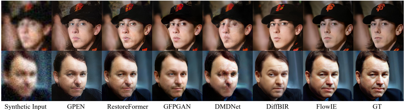
Figure 4. Qualitative comparisons on CelebA-Test. FlowIE generates plausible HQ results with enough details and high identity similarity even though input faces are severely degraded, while previous methods produce visible artifacts or inconsistent faces.
