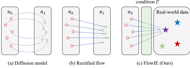
Figure 2. As shown in (a), diffusion models [16, 28] solve ODEs in curve trajectories. Differently, rectified flow [25], illustrated in (b), bridges one-to-one straight paths between two distributions, thereby reducing the inference steps. (c) Our proposed FlowIE applies the flow-based framework to real-world data and discards the massive data preparation process. We construct a many-to-one mapping that predicts straight paths to clean images from arbitrary noise in an elementary distribution with proper guidance.
