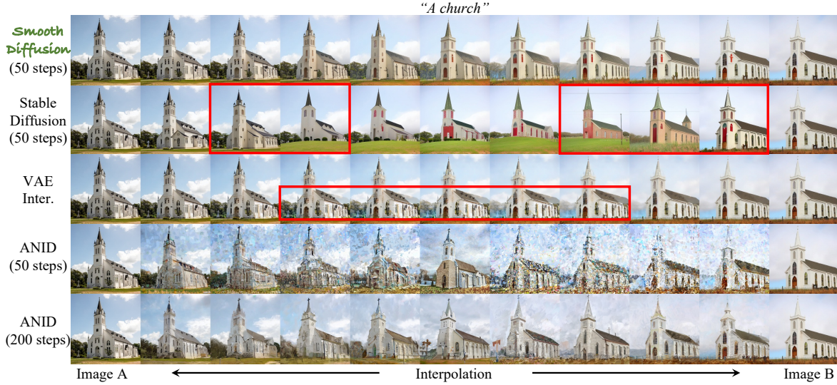
Figure 3. Image interpolation comparison results. For Smooth Diffusion and Stable Diffusion [62], real images (Image A and B) are inverted into latents using NTI [44]. We perform spherical linear interpolations between latents (also known as Stable Diffusion Walk [29]) and concatenate the resulting images as a transition sequence. VAE Inter. performs interpolations within the VAE space of Stable Diffusion. ANID [78] first adds noise to real images and subsequently denoises the interpolated noisy images using Stable Diffusion.
