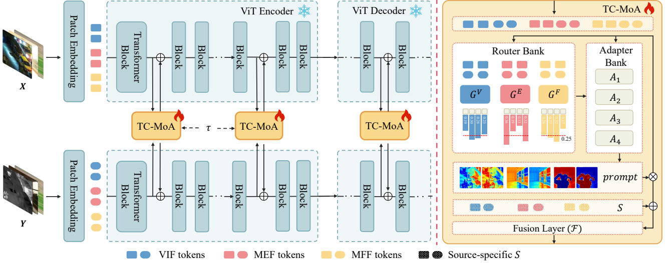
Figure 2. An overview of our proposed TC-MoA method. Our approach gradually modulates the fusion results by inserting TC-MoA into the frozen ViT backbone. TC-MoA generates task-specific prompt through a task-specific router bank and an shared adapter bank. The fusion layer utilizes prompt as scale and source-specific embeddings as biases to obtain fusion images.
