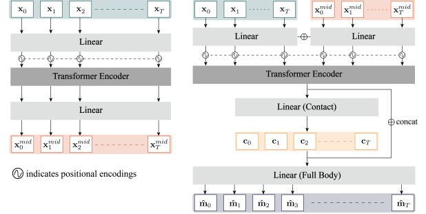
Figure 4. Network architecture of submodules \mathcal{F}^{end} (left) and \mathcal{F}^{body} (right) of \mathcal{F}_{est} .
