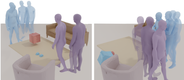
Figure 6. Qualitative results of multiple interaction generation: We present the outcomes of two distinct sequences within a living room environment, each defined by specific object geometries and a predefined configuration of 2 persons and 5 objects.
