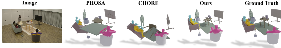
Figure 5. Qualitative comparisons of monocular multiple interaction capture on HOI-M 3 dataset with two state-of-the-art monocular HOI capturing methods PHOSA [65] and CHORE [52].
