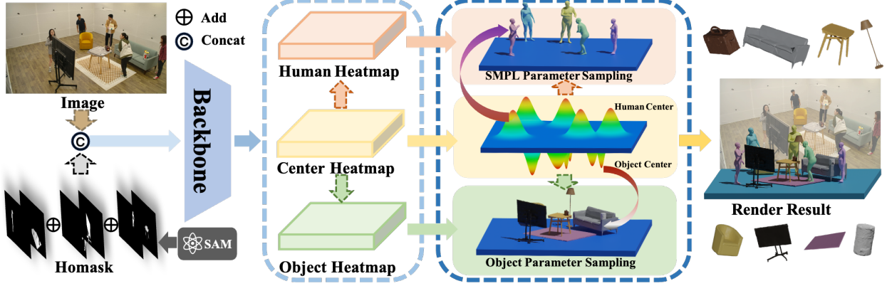
Figure 3. Monocular One-Stage Multiple HOI Capturing Pipeline. Given an input image, the pipeline predicts multiple maps: 1) the human-object center heatmap predicts the probability of the human’s root position or object’s center position, 2) the human mesh map contains the SMPL parameters and root depth, 3) the object mesh map contains the object 6D pose parameters and center depth. Through the sampling process, multiple humans and objects can be captured within a single forward process.
