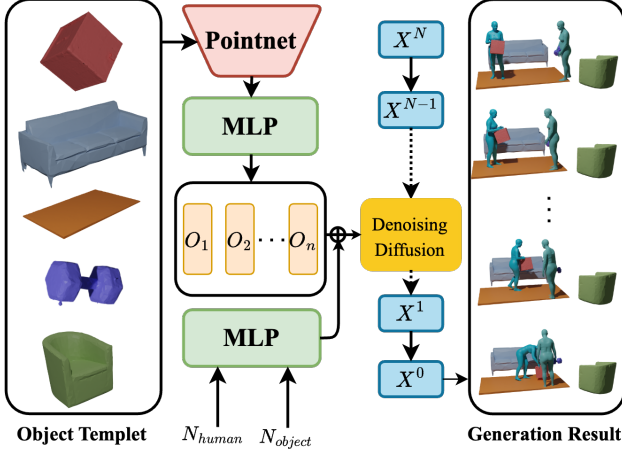
Figure 4. Multiple Interaction Generation Pipeline. Given multiple object geometry, we employ Pointnet to extract the geometry features and feed them forward with the features of the preset number of humans and objects using an MLP. The resulting features are then fed into a conditional diffusion model to generate multiple human-object interactions.
