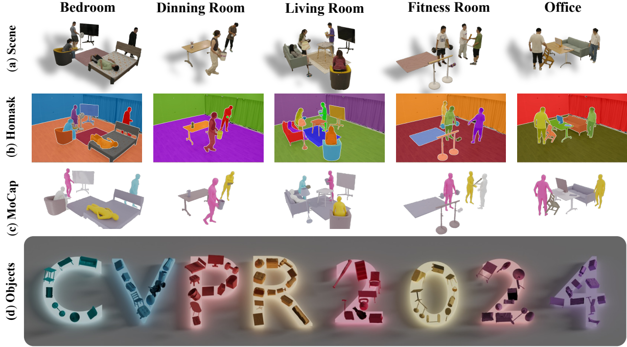
Figure 2. Overview of HOI-M 3 . (a) HOI-M 3 across five daily scenarios (Bedroom, Dining Room, Living Room, Fitness Room, Office), (b) annotated masks corresponding to each subject (human, object), (c) tracking of multiple humans and multiple objects, (d) significant number of pre-scanned object meshes.
