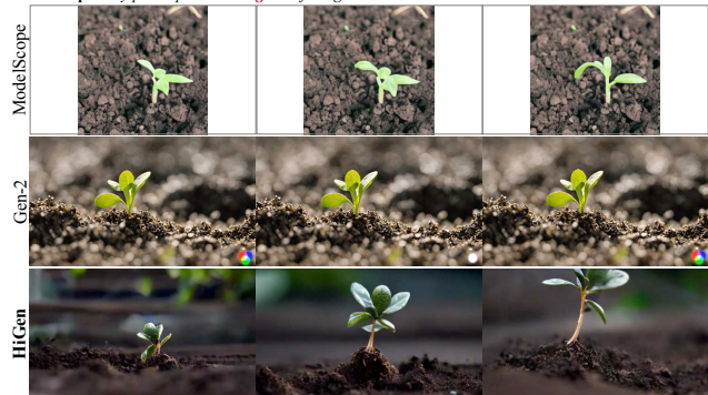
Figure 1. Visual comparison with ModelScopeT2V [53] and Gen-2 [10]. The videos generated by ModelScopeT2V exhibit noticeable motion but suffer from lower spatial quality. However, while Gen-2 produces realistic frames, they are mostly static with minimal motion. In contrast, the results of our HiGen demonstrate both realistic frames and rich temporal variations.
