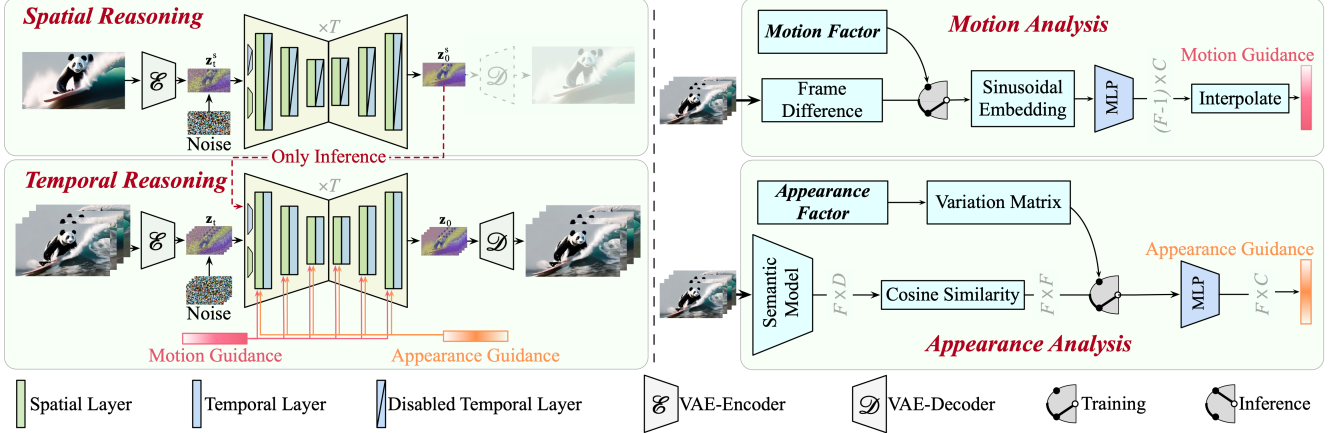
Figure 3. The overall framework of HiGen. Left : The structure-level spatio-temporal decoupling. Firstly, spatial reasoning is performed to obtain latent embeddings of spatial priors. Then, these spatial priors are used for temporal reasoning to generate videos. Right : The content-level motion-appearance decoupling. Motion analysis and appearance analysis refer to the calculations of motion and appearance guidance, respectively.
